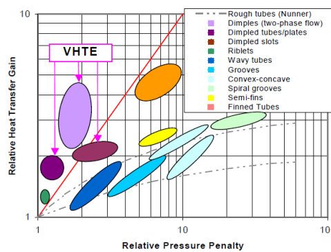
Figure 2. Effectiveness of different skin roughness technics [5].
