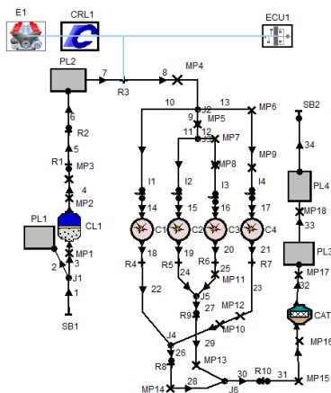
Figure 3. AVL Boost engine model for input data.
